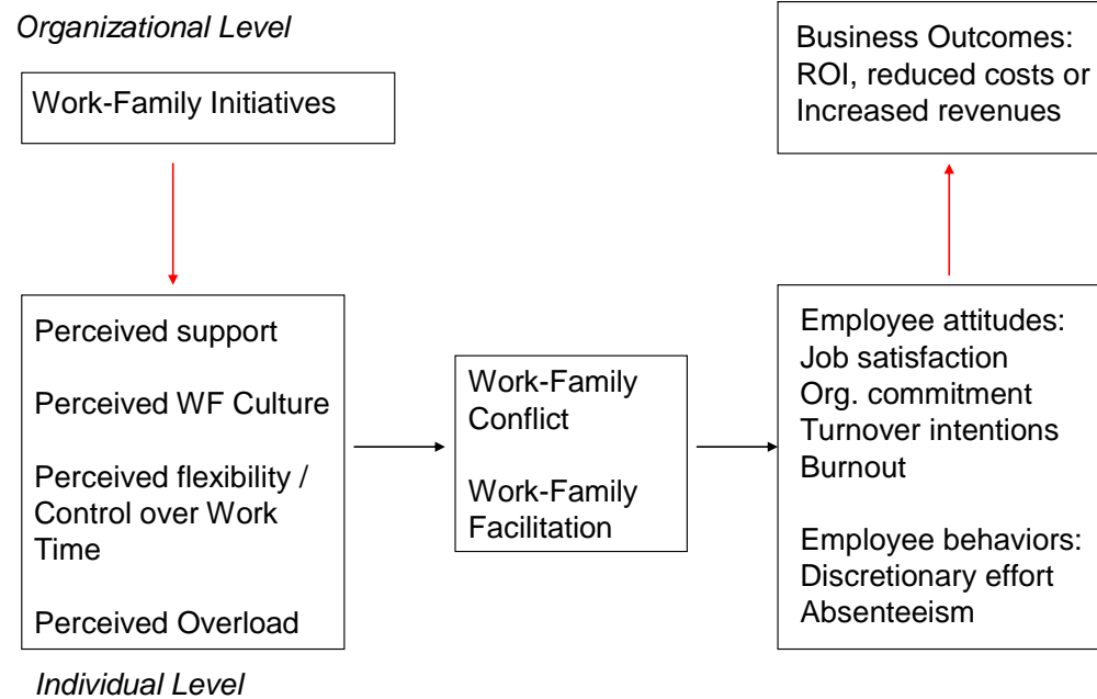
Figure 2: Conceptual Model
